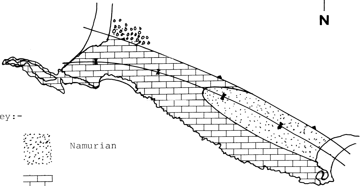
MAP OF RHOSILI & PORT EYNON, SHOWING THE EFFECT OF PLUNGE UPON THE OUTCROP OF THE NAMURIAN IN THE CORE OF THE PORT EYNON SYNCLINE
